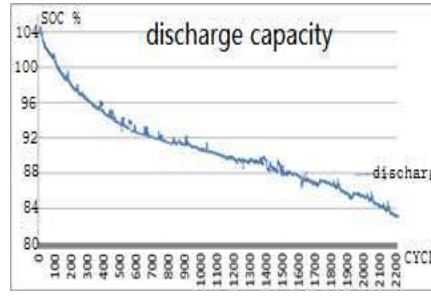
LFP battery discharge cycle at 0.5CA(100%DOD)
