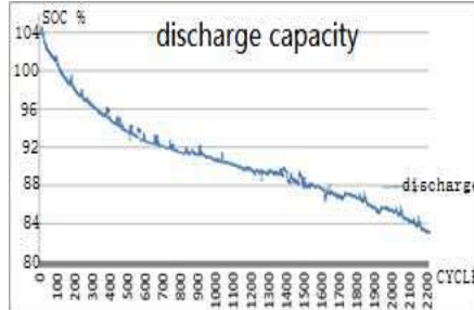
LFP battery discharge cycle at 0.5CA(100%DOD)
